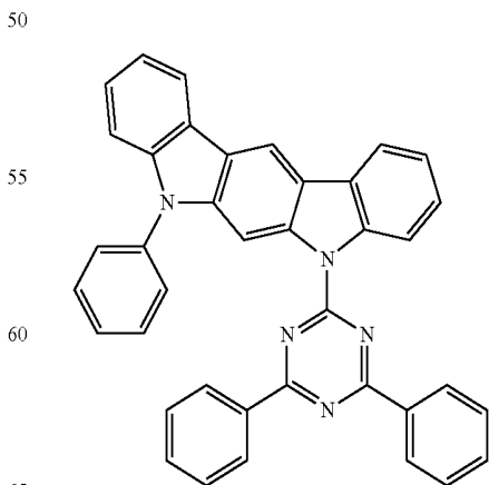
Compound EH14
