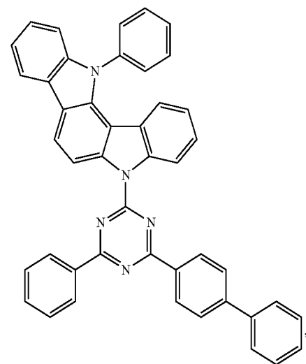
Compound EH32
