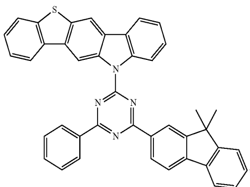
Compound EH14
