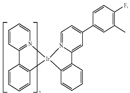
Compound 31
