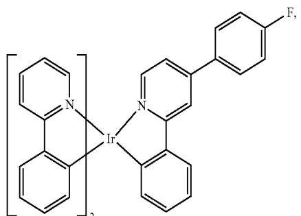
Compound 30
