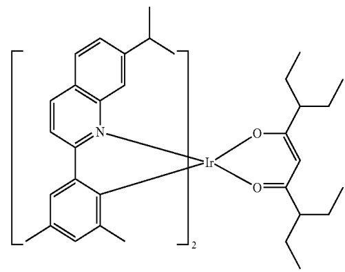
Compound E34
