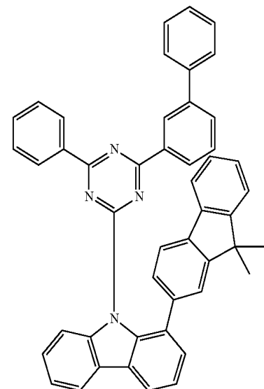
Compound H44
