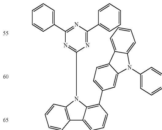
Compound H17
