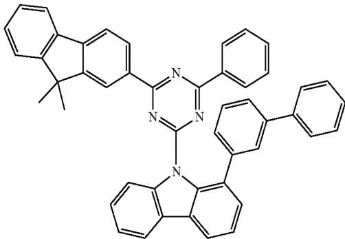
Compound H50
