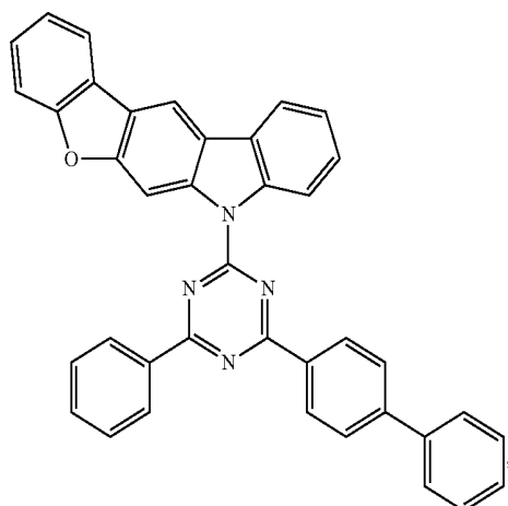
Compound EH25
