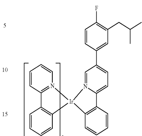
Compound 15
