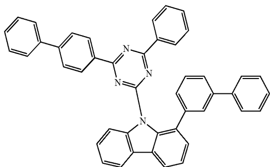
Compound H34
