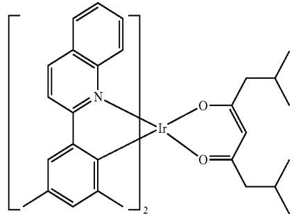
Compound E4
