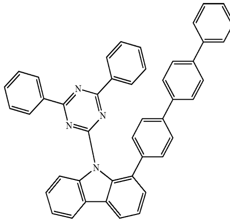
Compound H32
