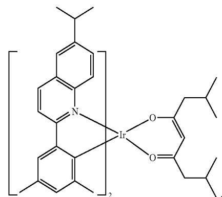
Compound E40
