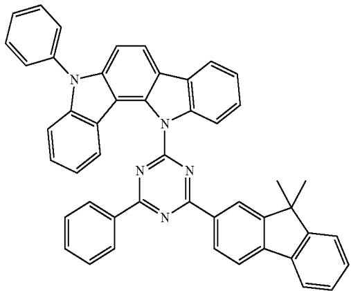
Compound EH43
