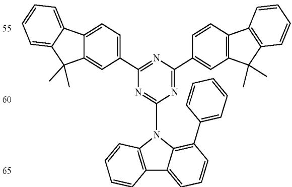
Compound H25
