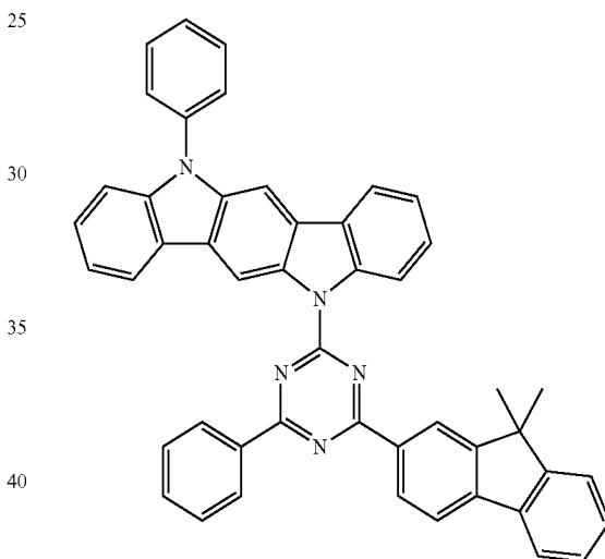
Compound EH16
