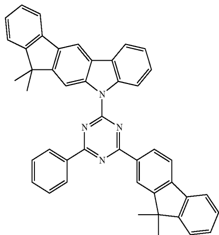
Compound EH29
