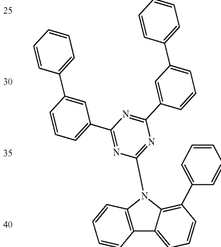
Compound H43
