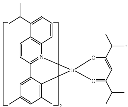
Compound E31
