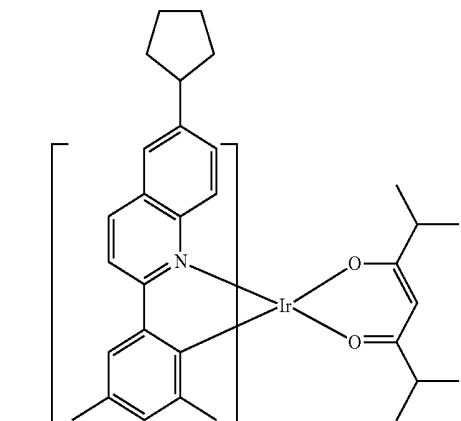
Compound E27
