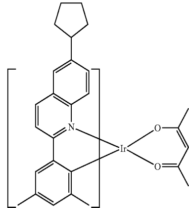
Compound E22
