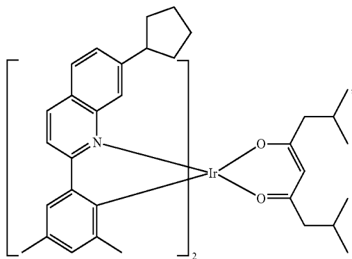
Compound E24
