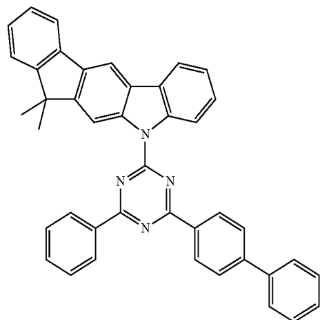
Compound EH28
