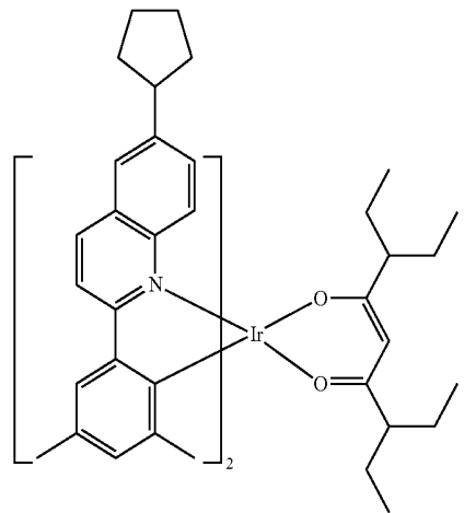
Compound E27
