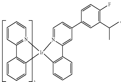
Compound 32
