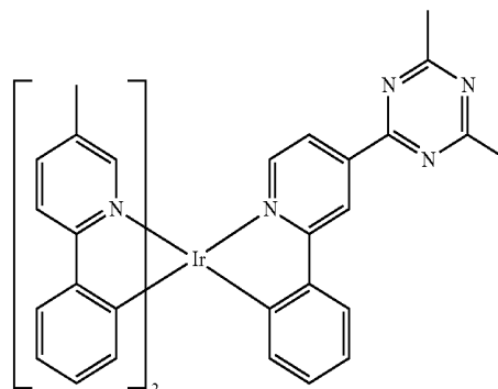
Compound 204
