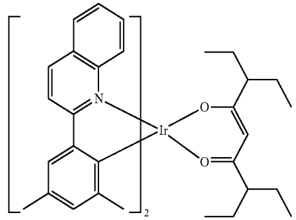
Compound E2
