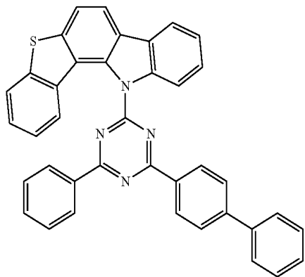
Compound EH44
