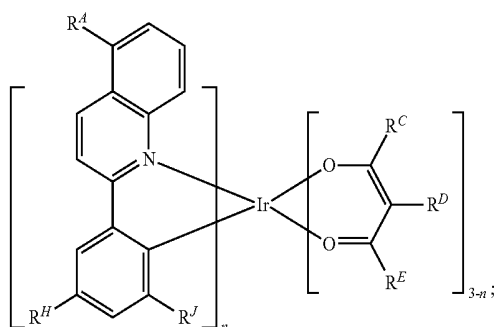
Formula IV
