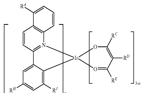
Formula IV
