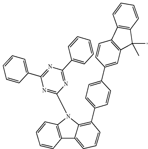
Compound H12
