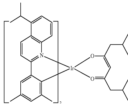
Compound E33
