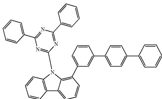
Compound H36
