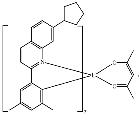
Compound E22
