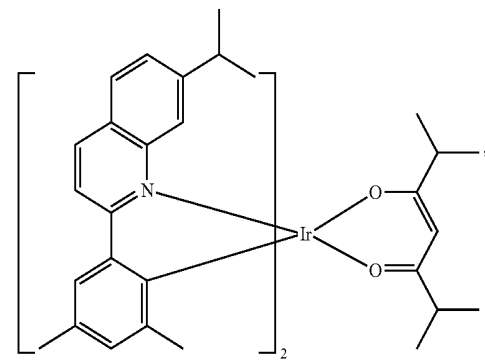
Compound E35
