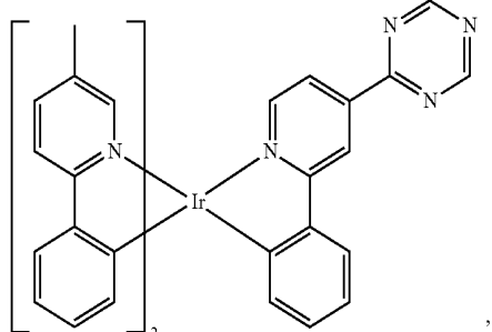
Compound 200
