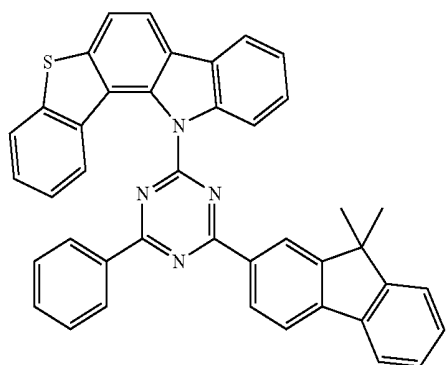
Compound EH45
