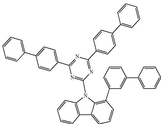
Compound H35
