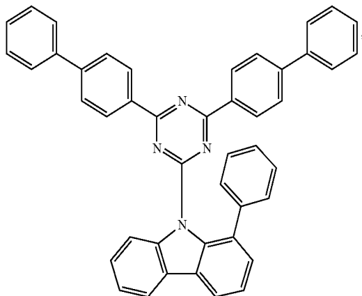
Compound H6
