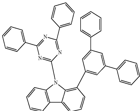
Compound H27
