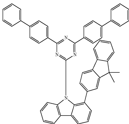
Compound H16
