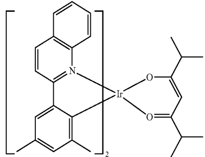
Compound H49
