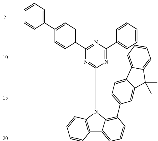
Compound H15
