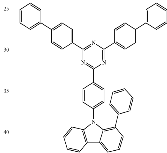
Compound H10
