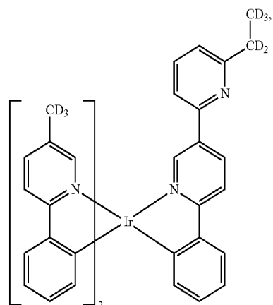
Compound 202
