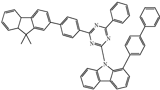
Compound H50
