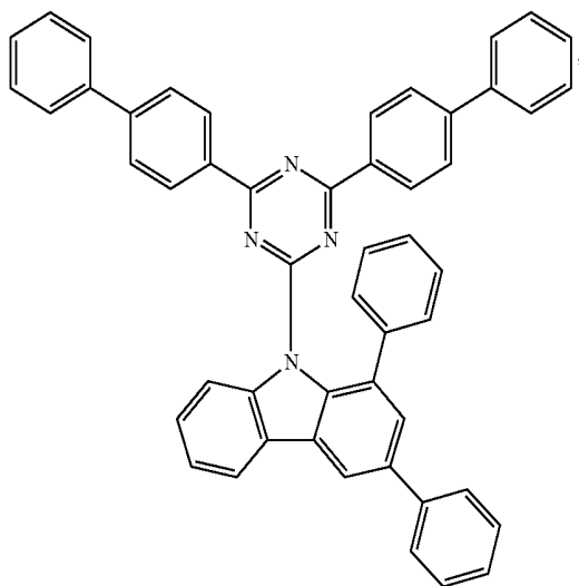
Compound H7
