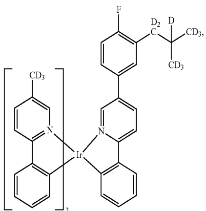
Compound 111
