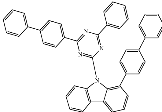
Compound H32
