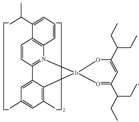
Compound E30
