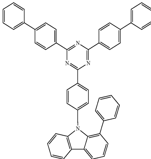
Compound H11
