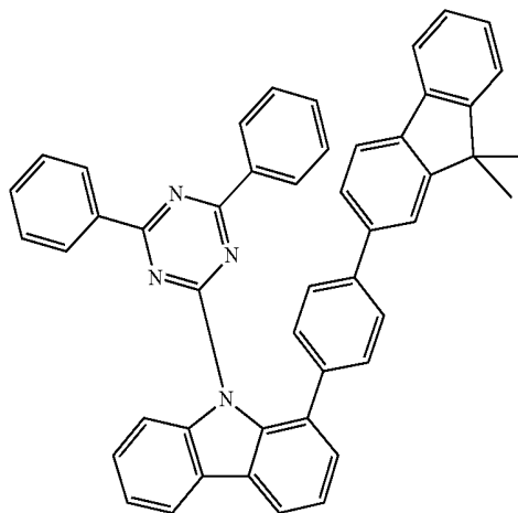
Compound H12
