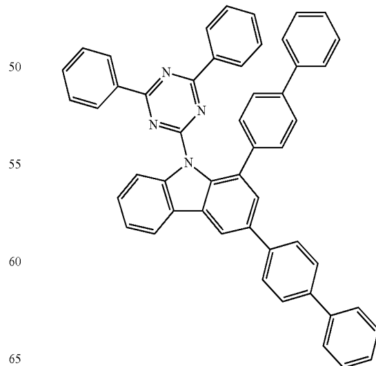
Compound H11
