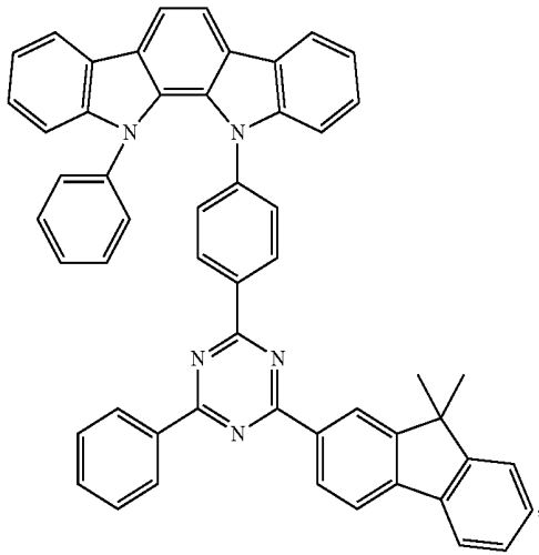
Compound EH50
