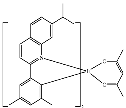
Compound E33
