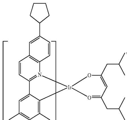
Compound E29
