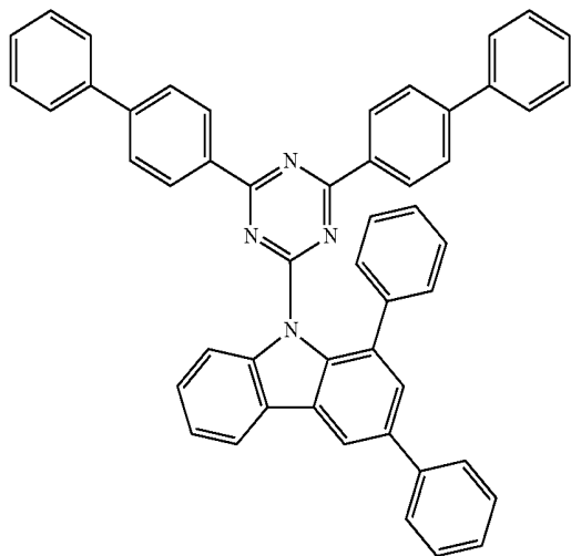
Compound H7
