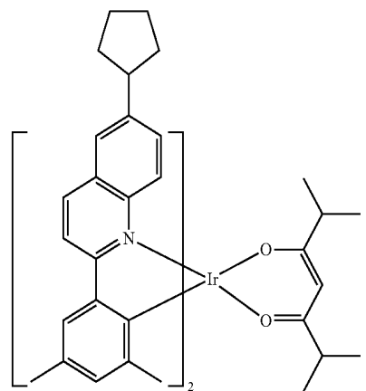
Compound E24
