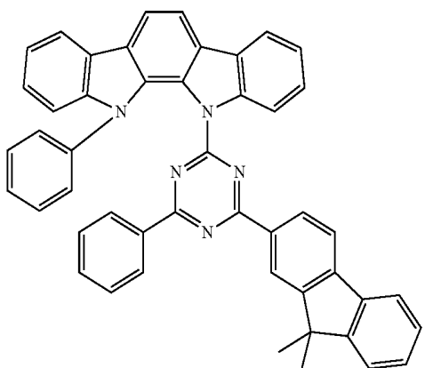
Compound EH6
