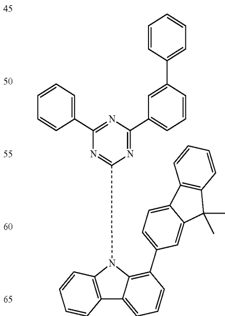
Compound H44
