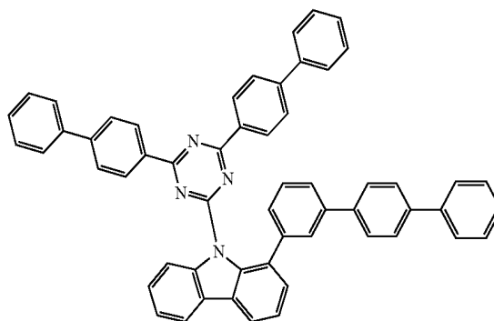
Compound H38
