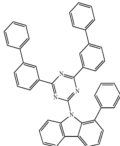
Compound H43
