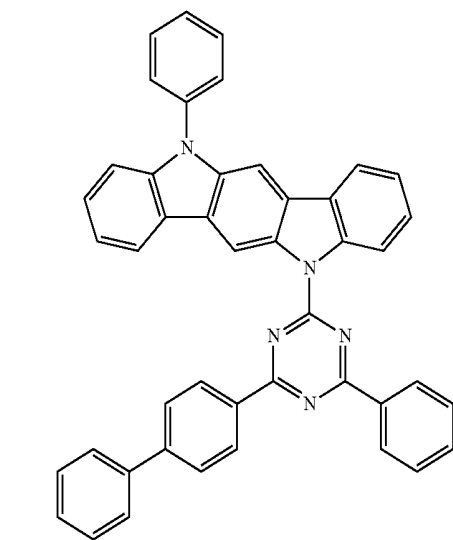
Compound EH9
